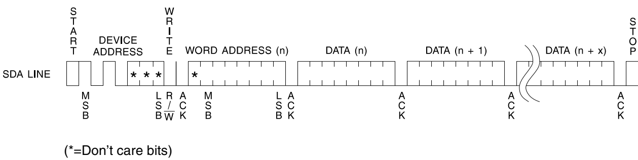
Figure 6. Page Write
